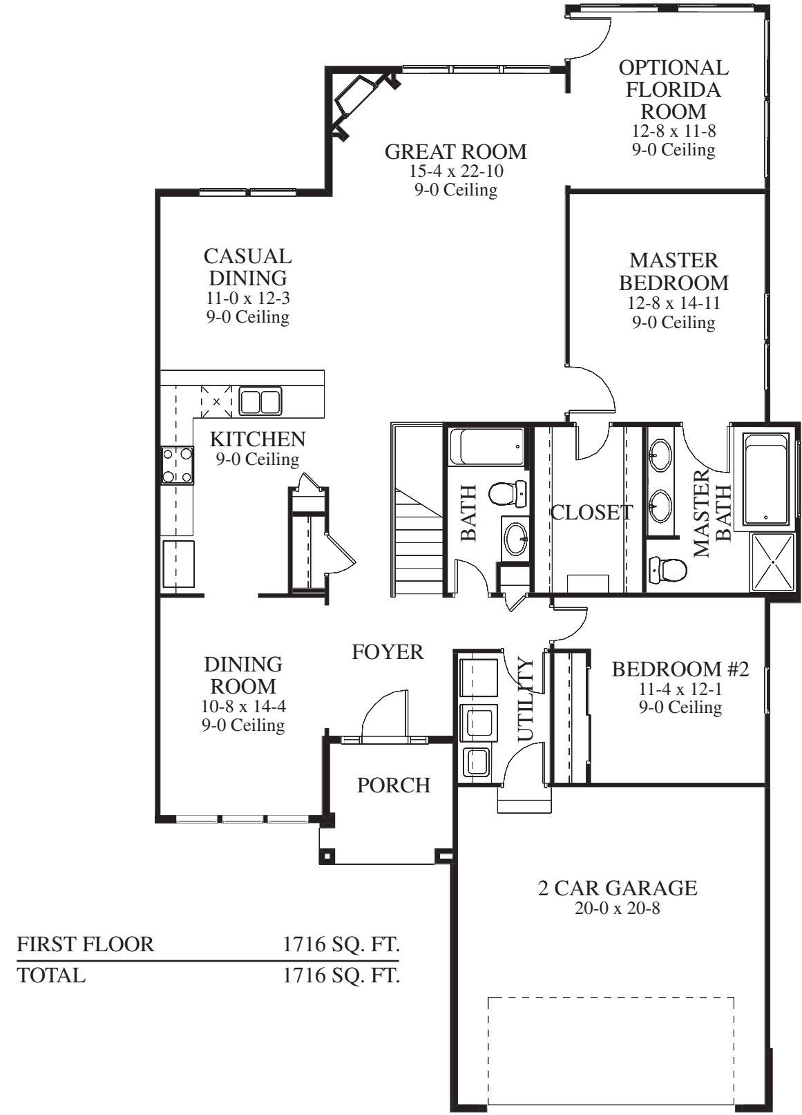
ASHTON RIGHT HAND FLOOR PLAN
