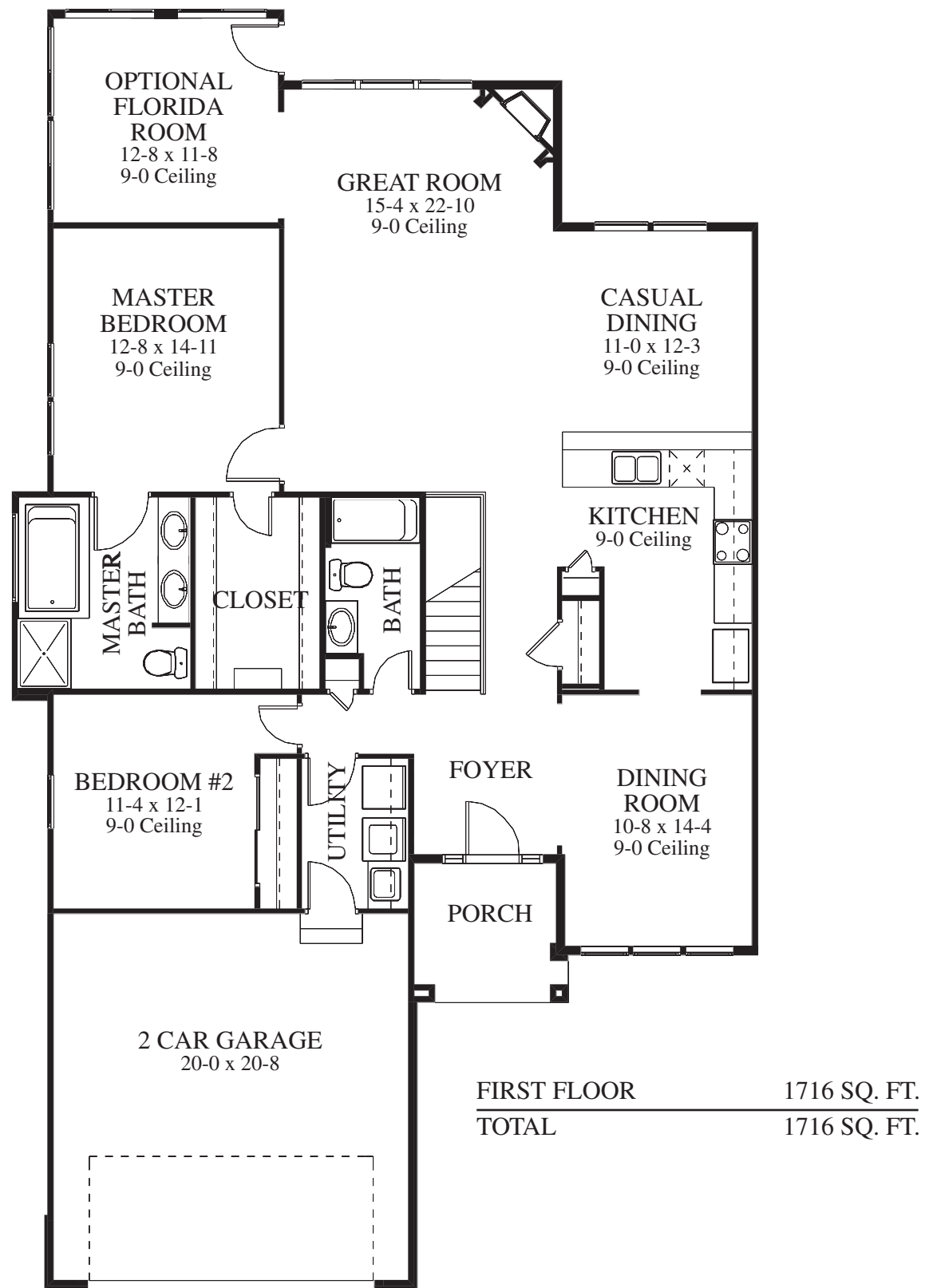
ASHTON LEFT HAND FLOOR PLAN
