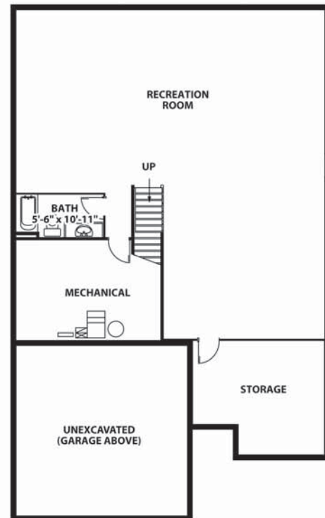
OPTION "ONE" FINISHED LOWER LEVEL PLAN TOTAL SQ. FT. PROPOSED: 1,561
